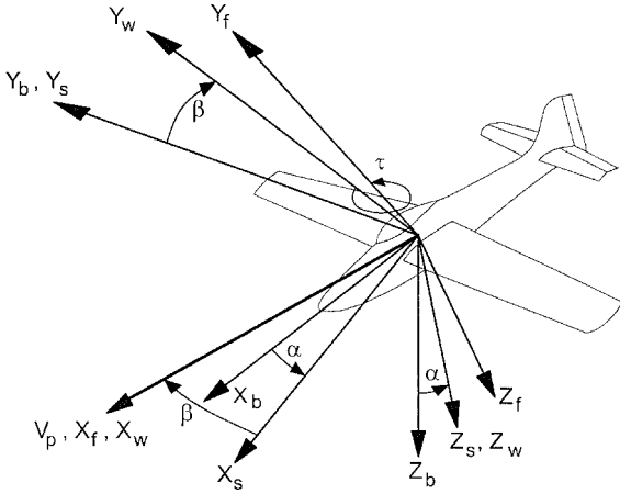
Fig. 2 Relationships between body, stability, wind, and Frenet axis systems.
