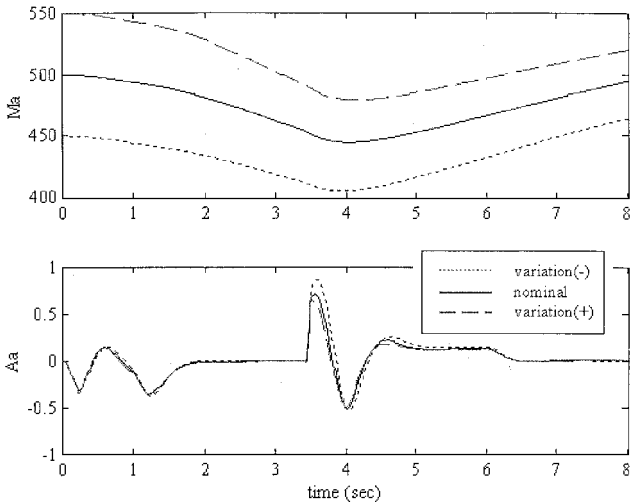
Fig. 10 Axial maneuver performance and axial agility time histories, test case 3.
